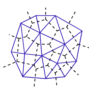
A Voronoi diagram (dotted lines) and its dual Delaunay triangulation (solid).
