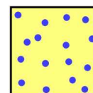
jittered
