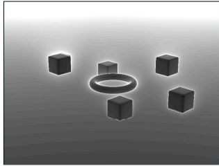
Distance field
