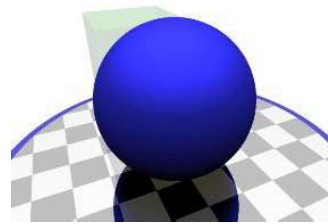
Difference
