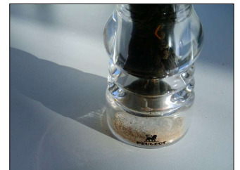
This is a photo of a real pepper-shaker. Note the caustics to the left of the shaker, in and outside of its shadow. Photo credit: Jan Zankowski
