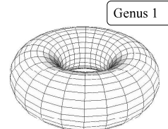
Genus 1
